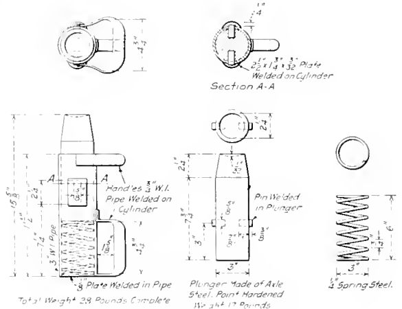
Staybolt Holder-On for Use with Pneumatic Hammer
